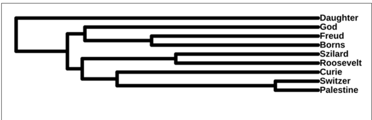
Figure 3. Rectangular dendrogram obtained from a stylometric analysis of Albert Einstein's letters, visualized with iTOL (Letunic, 2021).
