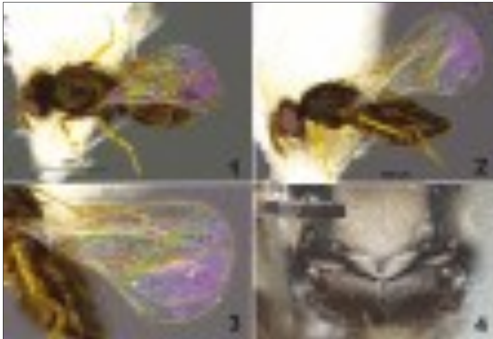
Figure 3. Tachinobia repanda Bouček (Hymenoptera: Eulophidae). (1) Female, dorsal view; (2) Female lateral view; (3) Forewing; (4) Lower part of scutellum+dorsellum+propodeum.
