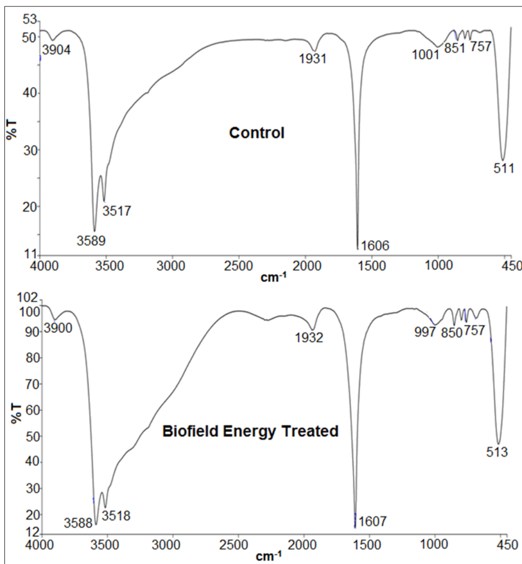
Figure 4. FT-IR spectra of the control and Biofield Energy Treated zinc chloride.
