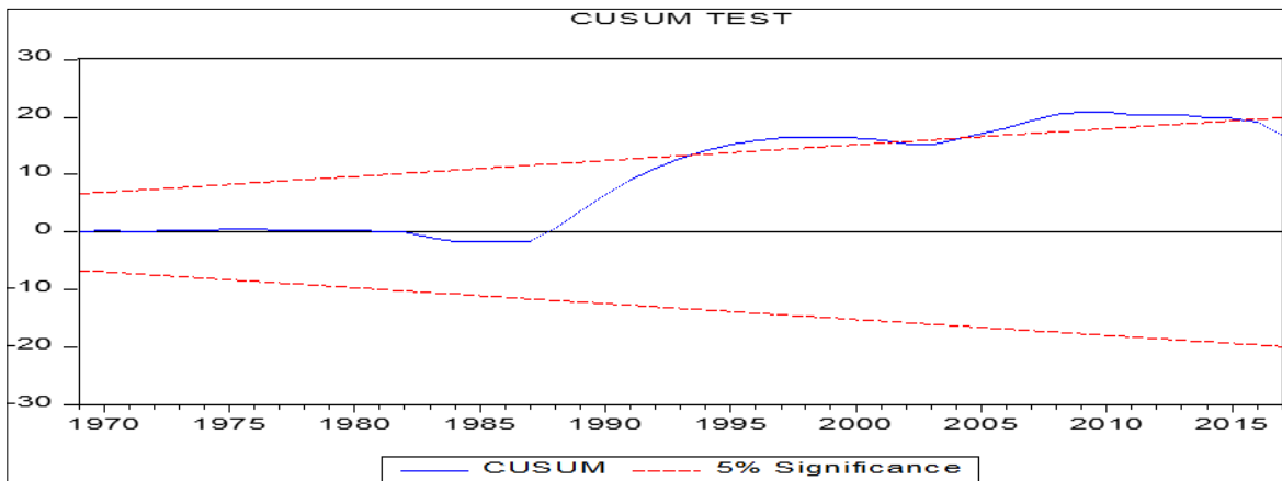
Figure 8. CUSUM test
