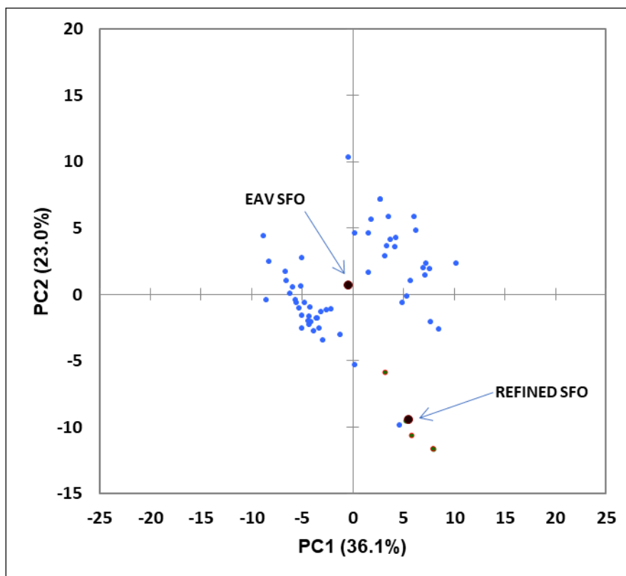
Figure 3. PCA scores plot of PC2 versus PC1 for the ^1\text{H} NMR spectral profile ISB dataset of EAV (blue) and refined, EU-available SFO products (red). The percentage contributions of each PC to the total model variance are provided in brackets for each axis label. Cluster centroids for each SFO classification are indicated in black.
