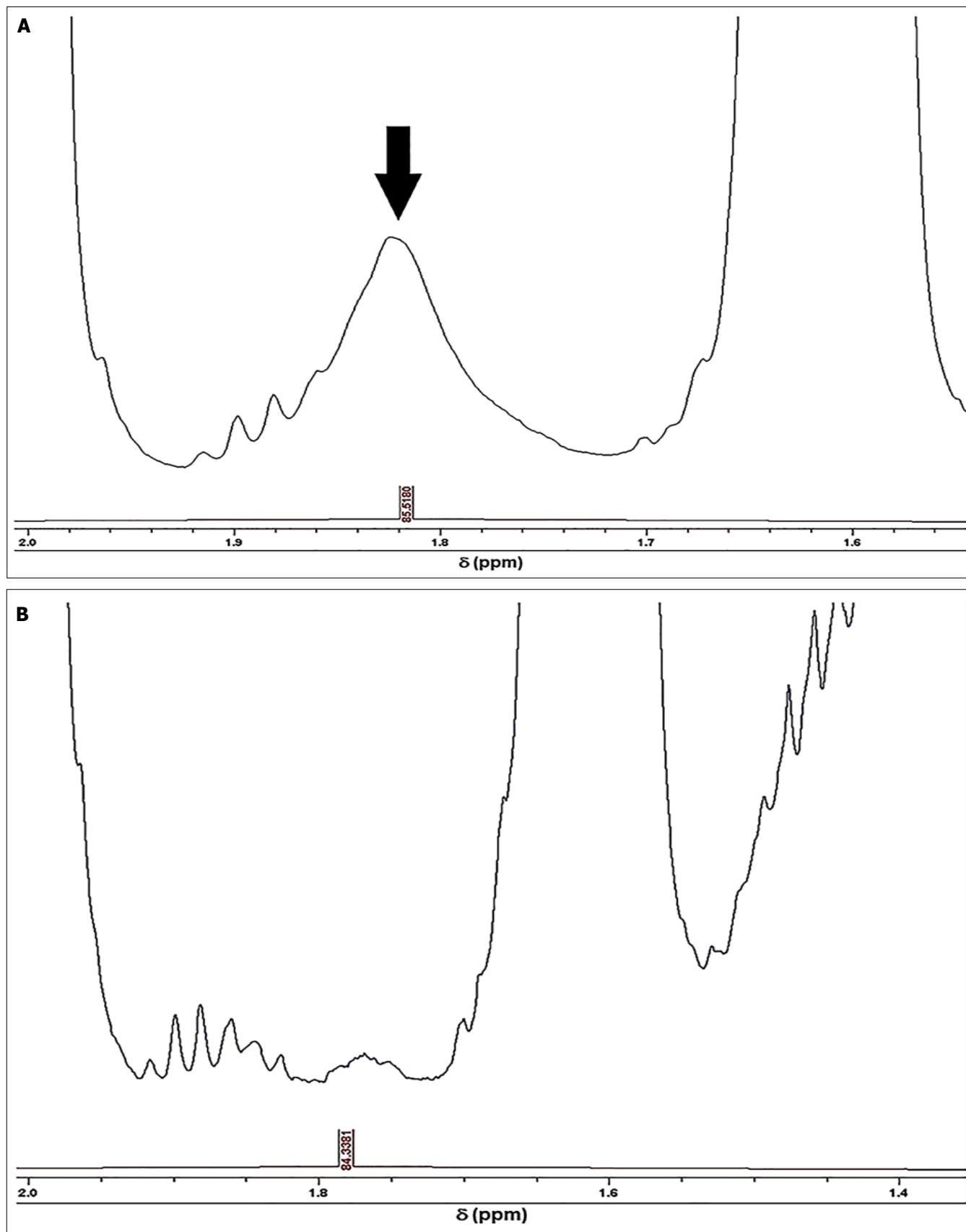
Figure 2. Expanded 1.54-2.00 and 1.35-2.00 ppm regions of the ^1\text{H} NMR profiles of (a) EU-available refined, and (b) EAV SFO products respectively. The major 1.79-1.83 ppm ISB marker resonance for the refined SFO products is indicated in (a).
